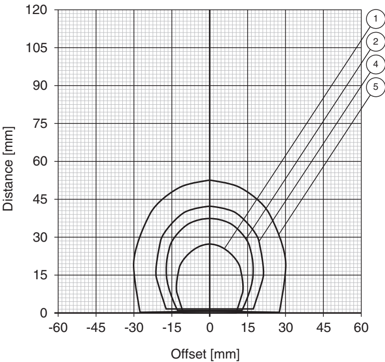
Writing range in air IPC03-30..
