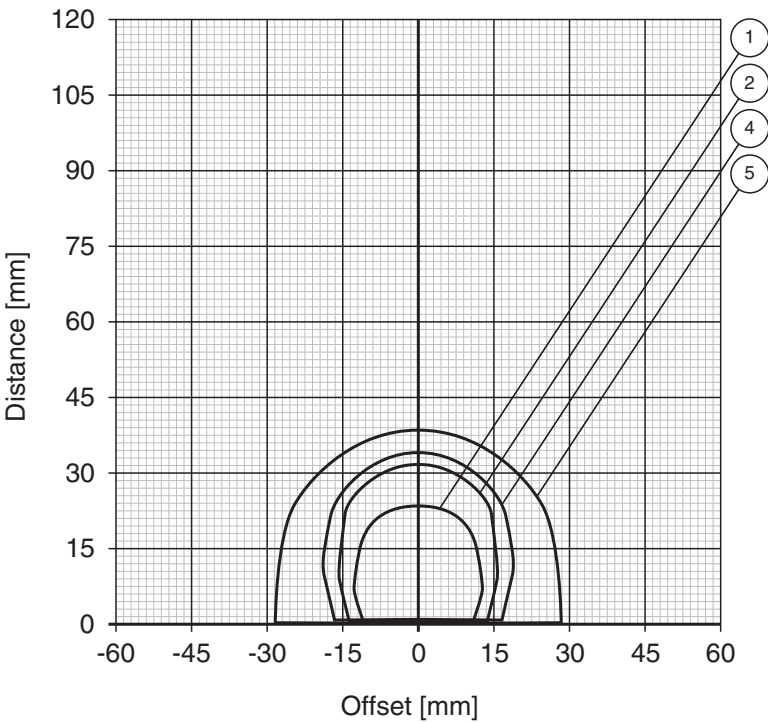
Writing range on aluminium IPC03-30..
